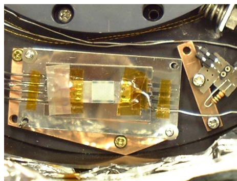
図 7.14: ADR's SQUID shield mounted in 02/12/25.
