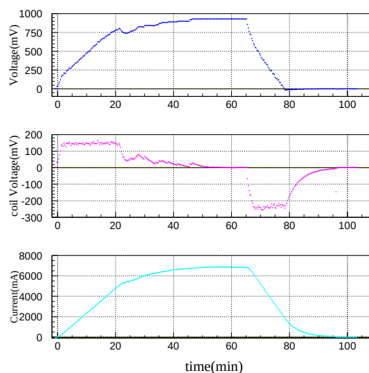
図 4.6: Adiabatic Demagnetization result in 02/06/28. Voltage and Current.
