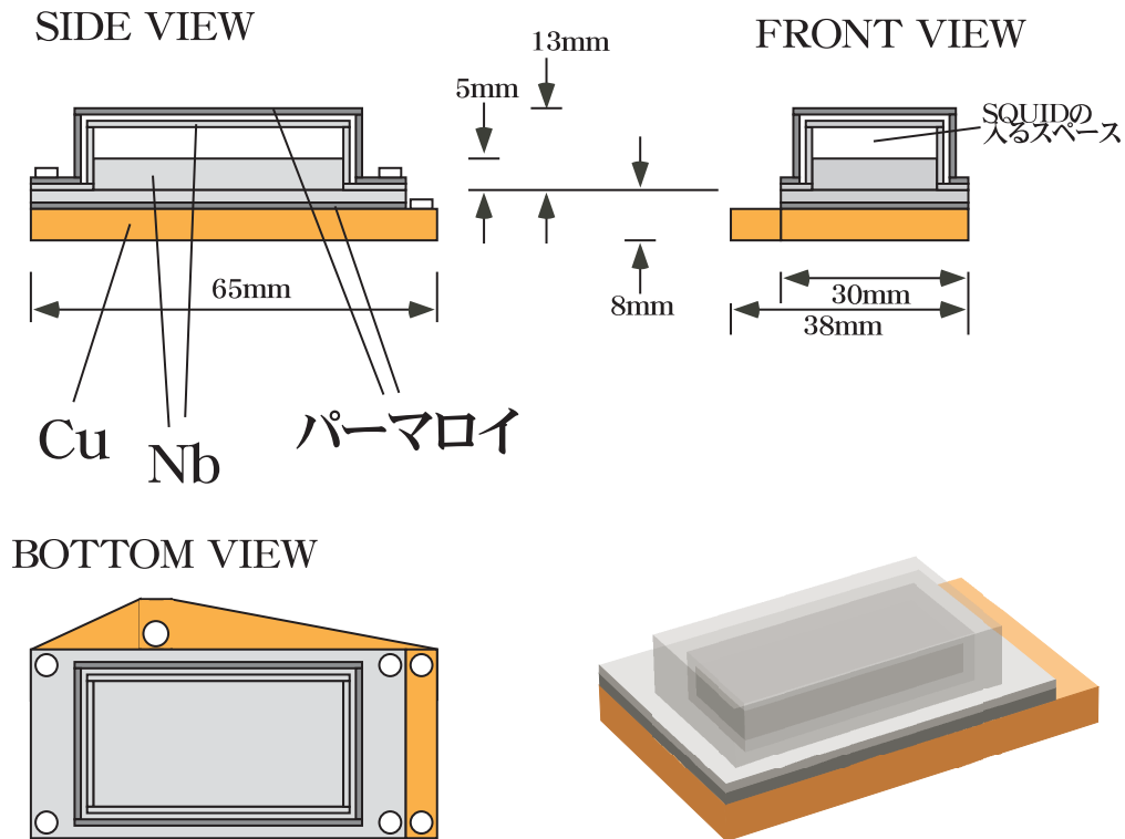
図 7.11: ADR's SQUID shield assembly.
