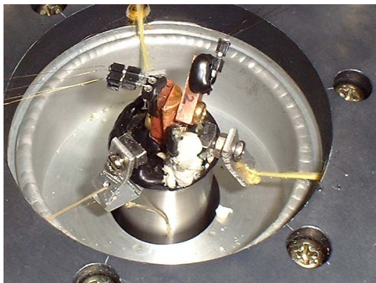
図 4.16: figure of saltpill no2. after experiment
