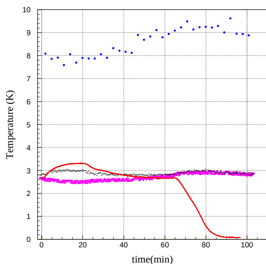
図 4.5: Adiabatic Demagnetization result in 02/06/28.
