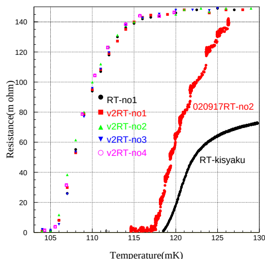
図 6.10: RT results in 02/09/04 and 02/09/17
