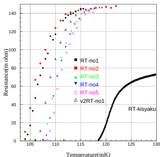
図 6.9: RT results in 02/08/09
