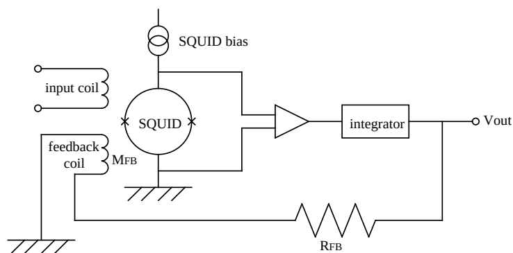
図 2.9: Flux-locked loop
